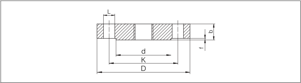
Fig. 21: Dimensions - JIS flange (Regular Flange)
